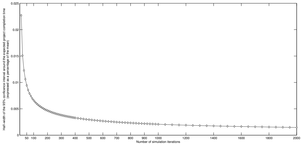
Figure 12: Average half-width of the 95 percent confidence interval around the expected project completion time
